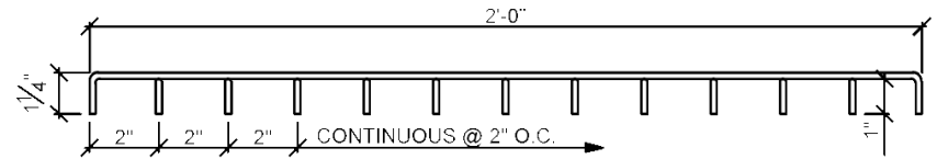
SECTION VIEW
